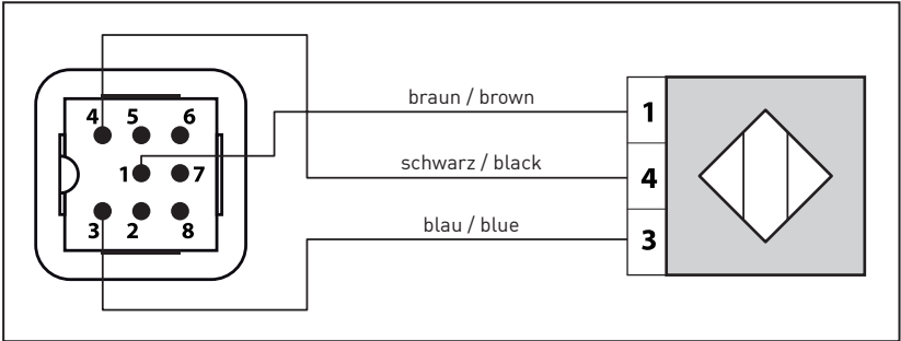
Fig. 10-5: Circuit diagram for connecting the Klübermatic ECOSY Control sensor
